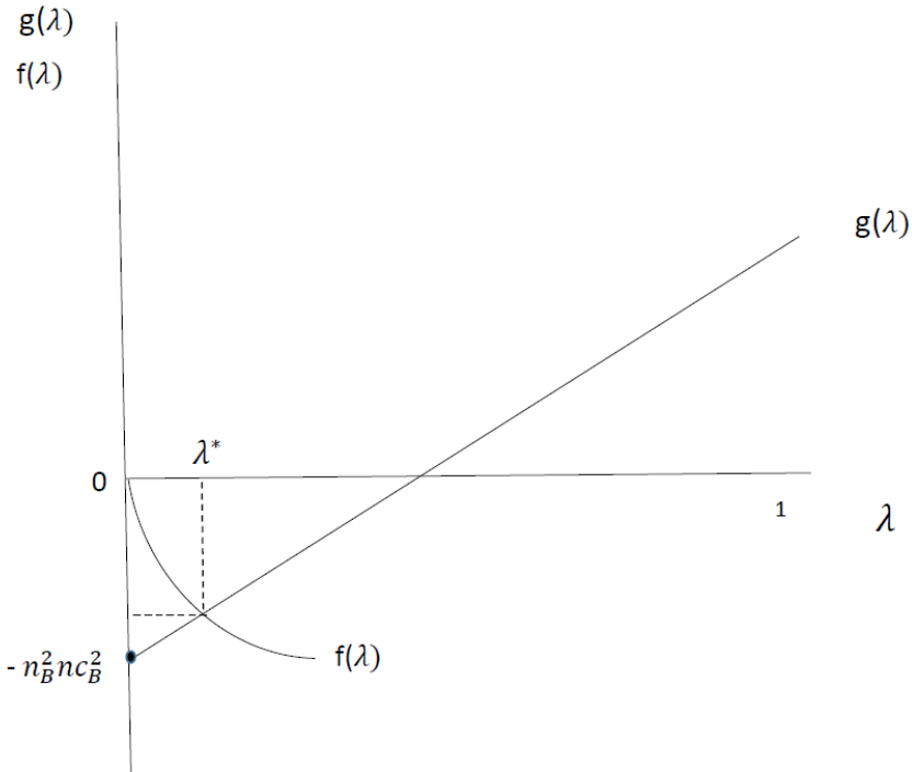
FIGURE 3 VALUE OF \lambda^* AT EQUILIBRIUM
