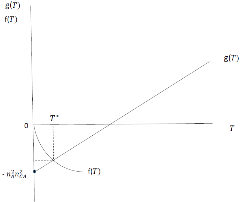
FIGURE 2 VALUE OF T^* AT EQUILIBRIUM
